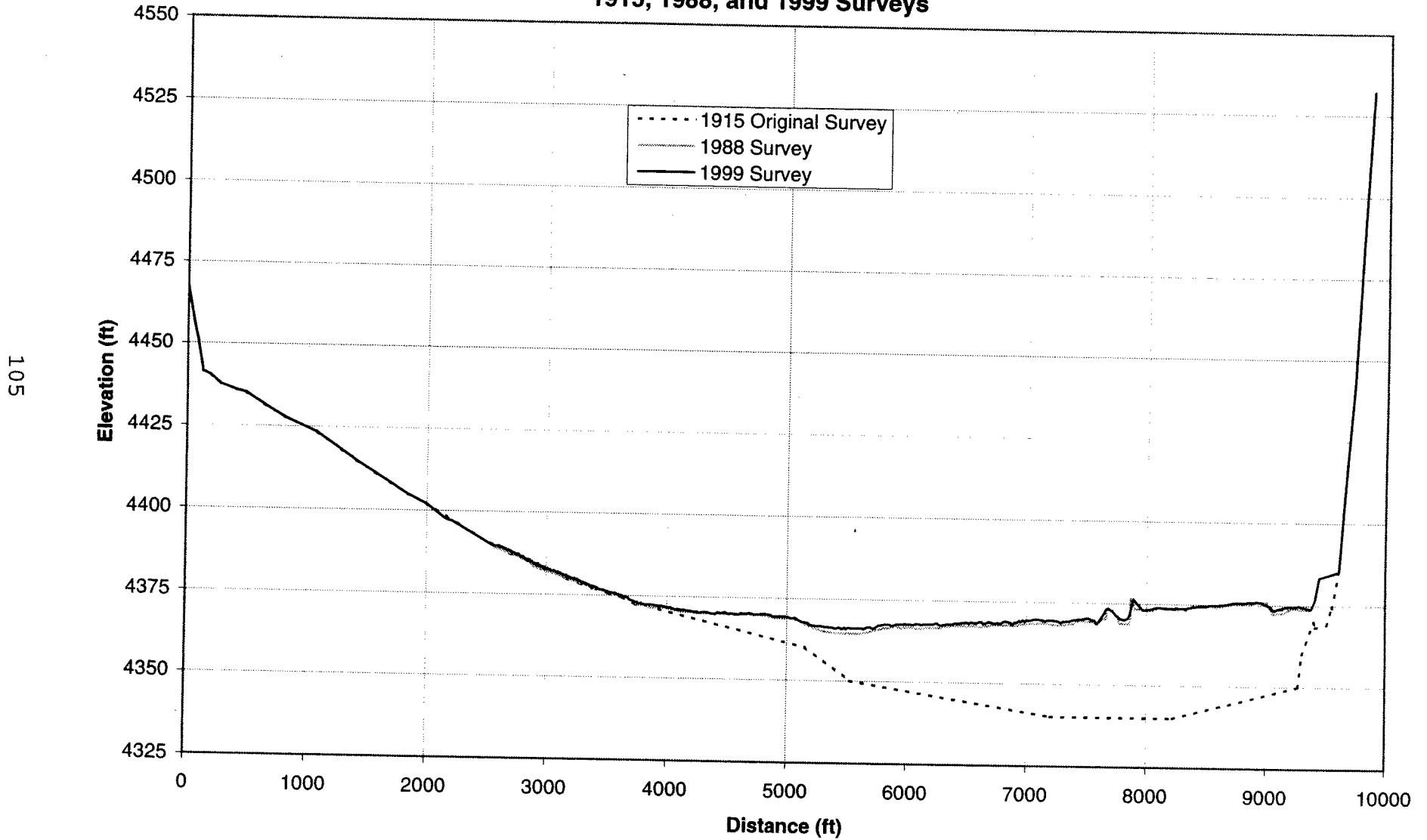
Figure 71. - Sedimentation range profiles for 1915, 1988, and 1999, range 39.
