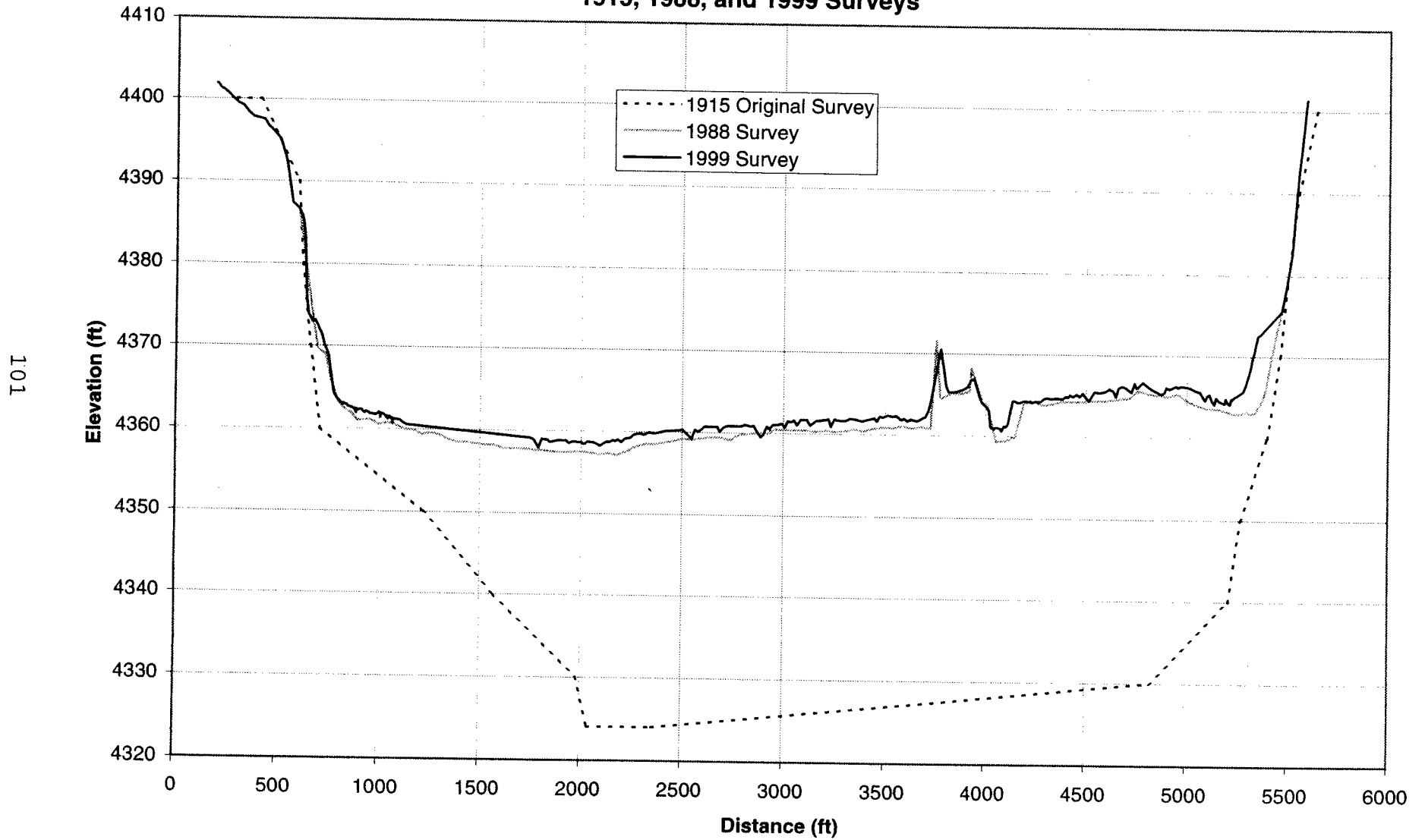
Figure 67. - Sedimentation range profiles for 1915, 1988, and 1999, range 43.
