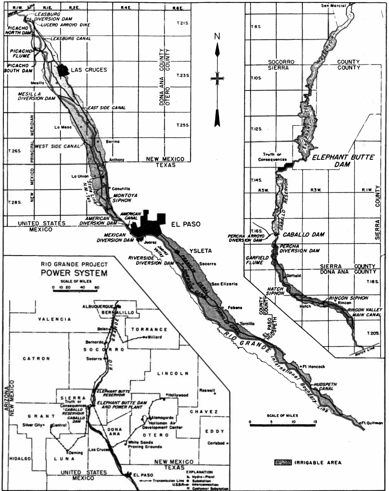
Figure 1 - Elephant Butte Reservoir location map.
