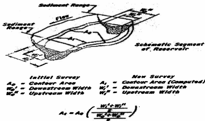
Figure 102 - Width adjustment method for revising contour areas
